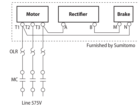
Figure 5.39 Normal Brake Action, 575V
