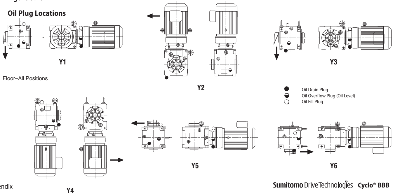
Figure 5.45 Oil Plug Locations
