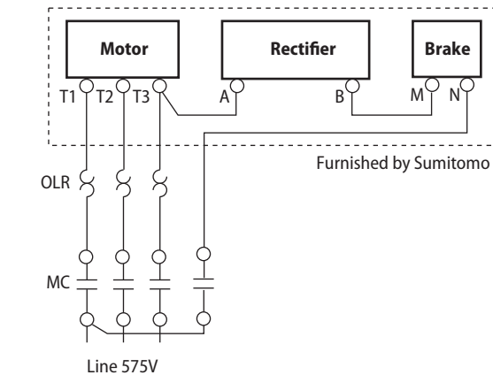
Figure 5.40 Fast Brake Action, 575V
