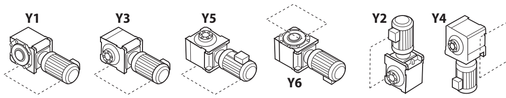
Mounting Positions
