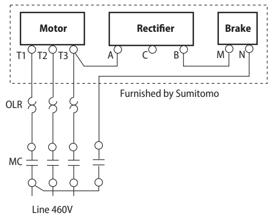
Figure 5.38 Fast Brake Action, 460V
