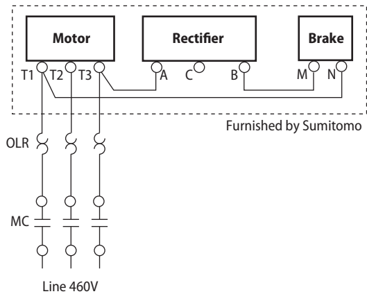
Figure 5.37 Normal Brake Action, 460V
