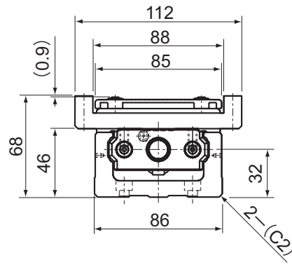
B-B cross section
