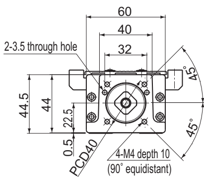
A arrow view
