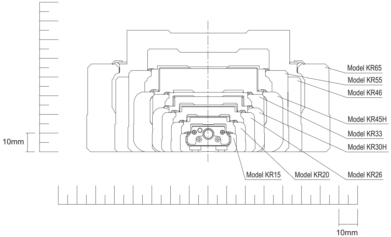
Fig.5 Cross Sectional Drawing
