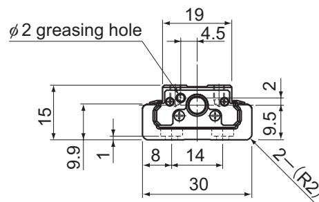
B-B cross section
