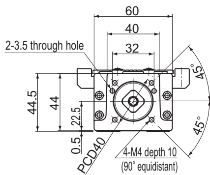
A arrow view
