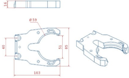
HSK F63
